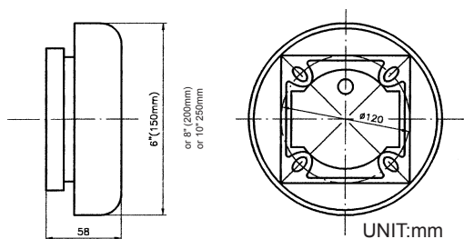
CB-6 CB-8 and CB-10 (6, 8, 10 inch bell)
