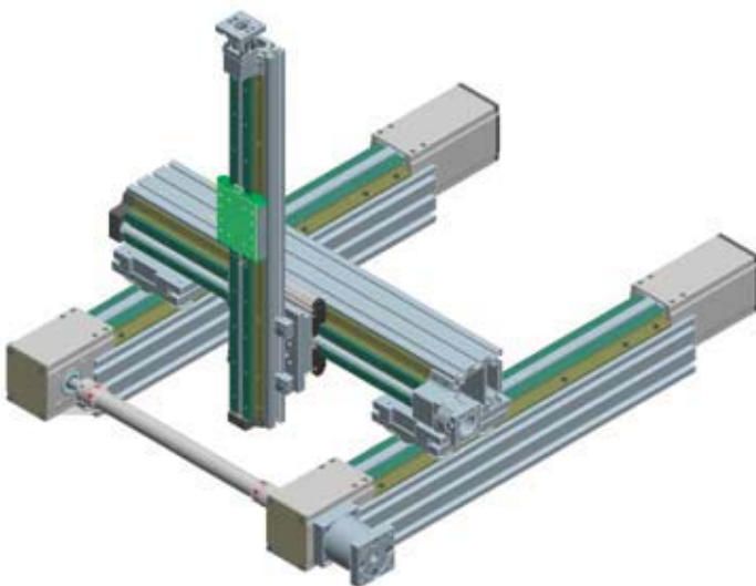
X-Y-Z Multi-Axis Arrangement
