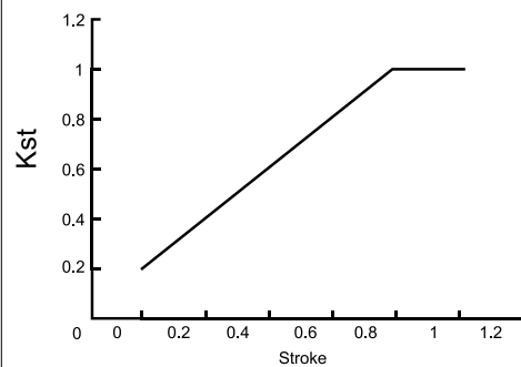
Short stroke factor diagram
