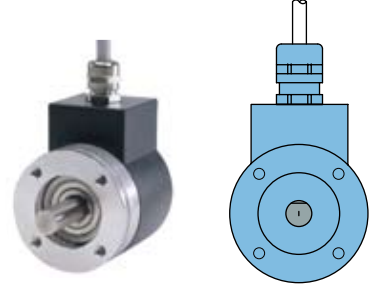
SERVO MOUNT #2 10-32 UNF-2B 0.25 DEEP 4X 90° Ø1.625 B.C.
