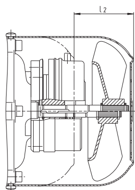
Motor type 13.750 Brake type BFK458-06
