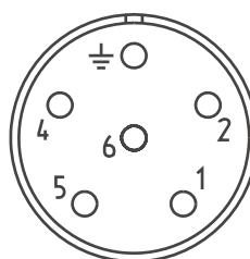
Power connector
