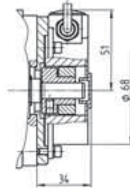
Motor type 13.120 Tacho type TD3
