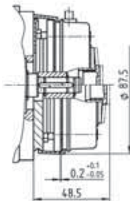
Motor type 13.120 Brake type BFK458-06
