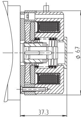
Motor type 13.120/13.710
