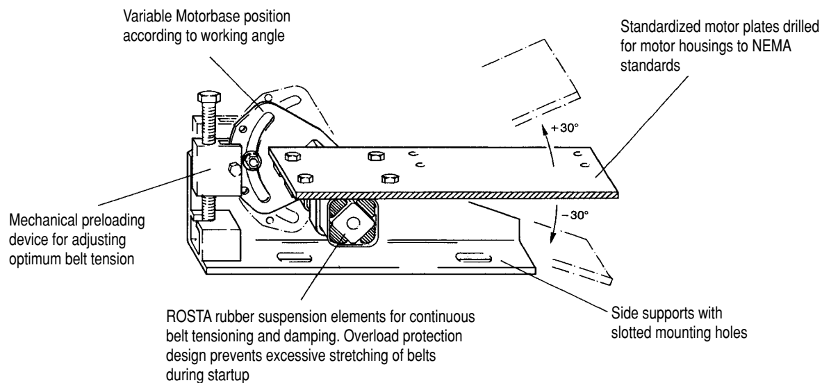
Illustration of Motorbase for 7½ to 75 HP Motors
