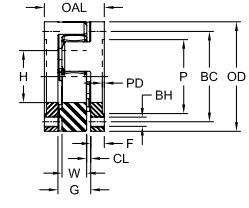
CJDSF Design
