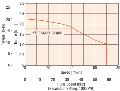
AR24 Gear Ratio 100
