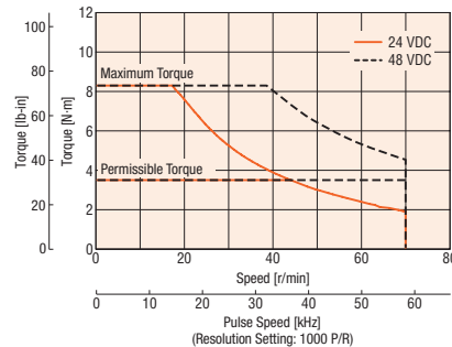
AR46 Gear Ratio 100
