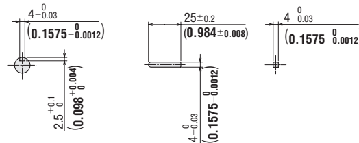
A-A Parallel Key (Included)
