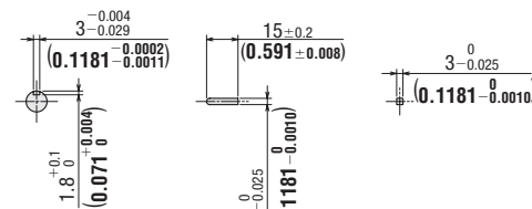
A-A Parallel Key (Included)
