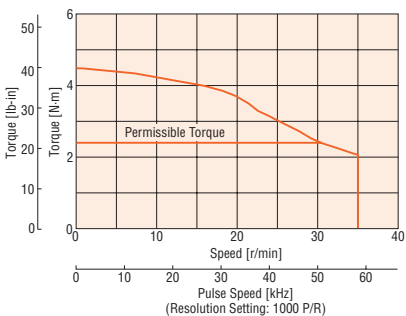
AR24 Gear Ratio 100
