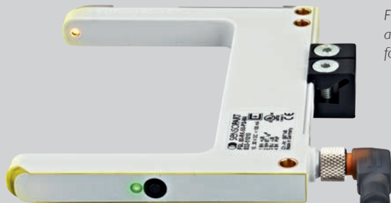
FGL with mounted MBD-S94 bracket and easily visible Indicator LEDs on the fork edge.
