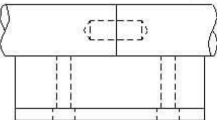
DOWEL JOINED SHAFT SUPPORT ASSEMBLIES
