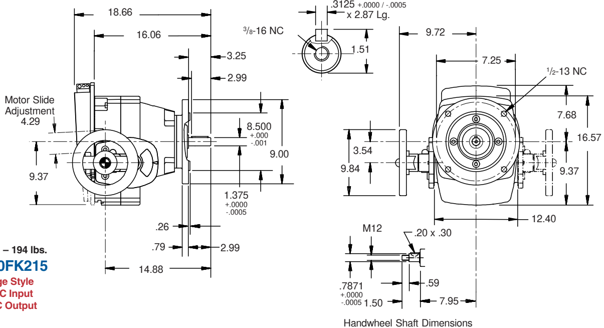
Handwheel Shaft Dimensions
