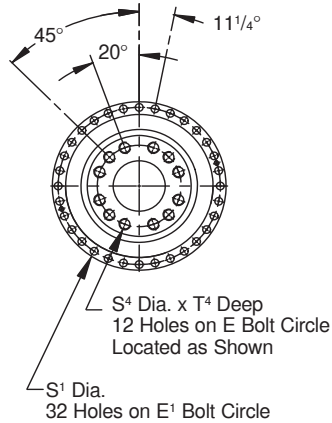
PHQA9/PHQA10 OUTPUT SIDE
